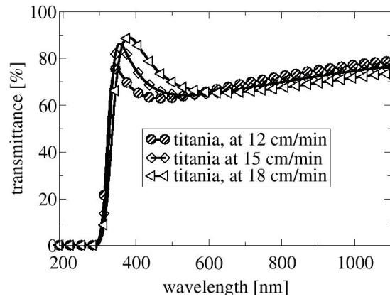
Figure 7: Transmittance spectra of \text{TiO}_2 film prepared with different withdrawal velocities
