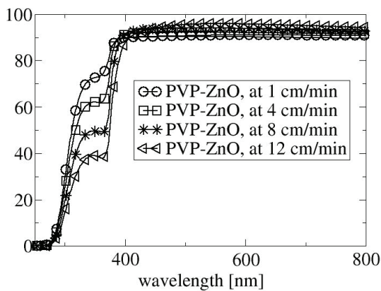
Figure 2: Transmittance spectra of PVP-ZnO films prepared with different withdrawal velocities
