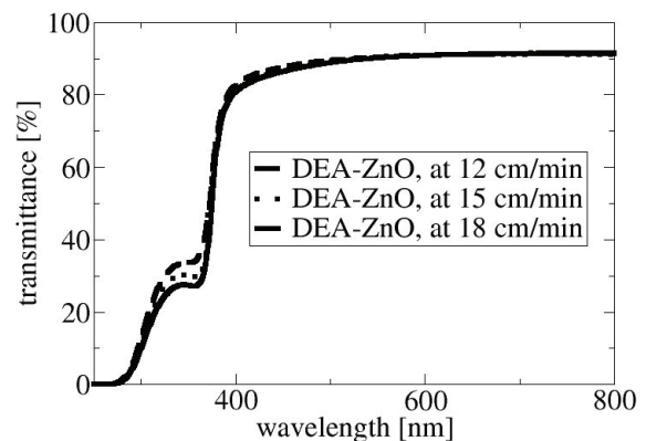
Figure 4: Transmittance spectra of DEA-ZnO films prepared with different withdrawal velocities
