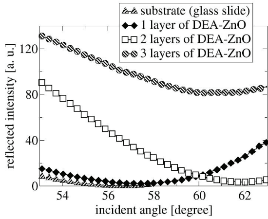
Figure 6: Results of SAR measurements on DEA-ZnO films containing 1, 2 and 3 layers
