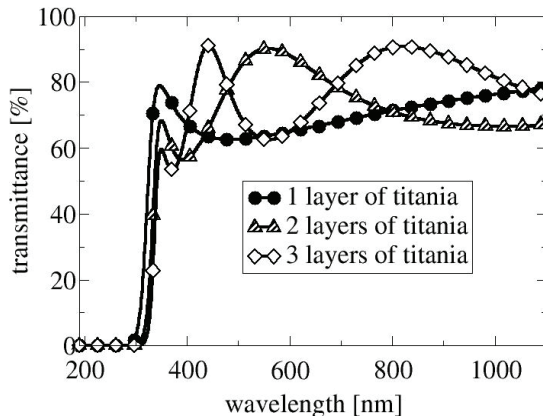
Figure 8: Transmittance spectra of TiO 2 films containing 1, 2 and 3 layers
