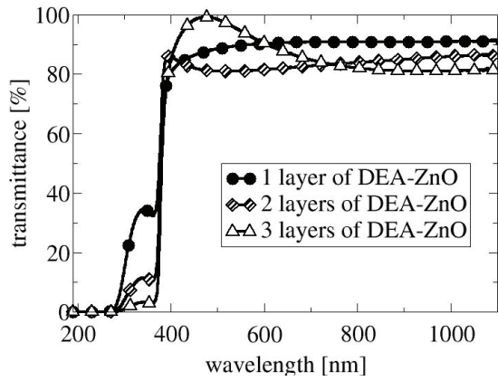
Figure 5: Transmittance spectra of DEA-ZnO films containing 1, 2 and 3 layers
