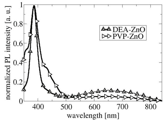
Figure 10: Photoluminescence spectra of DEA-ZnO and PVP-ZnO films
