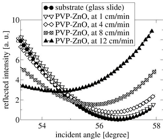
Figure 3: Result of SAR measurements on PVP-ZnO films prepared with different withdrawal velocities
