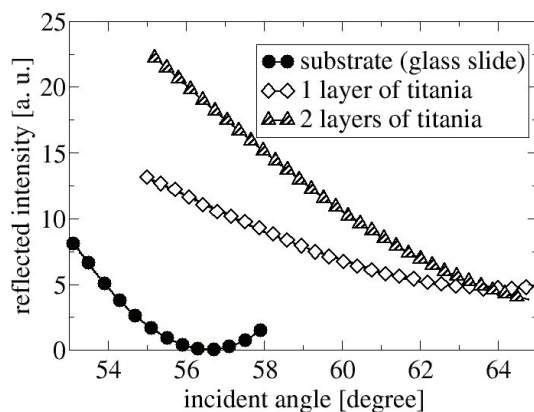
Figure 9: Results of SAR measurements on TiO 2 films containing 1 and 2 layers
