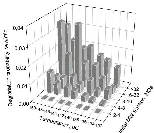
Fig. 7. Degradation probabilities of different molecular weight fractions at various treatment temperatures
