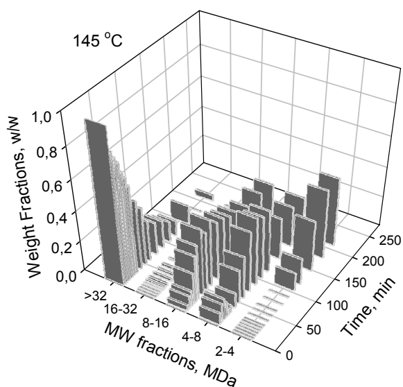
Fig.4. Evolution of weight fractions of the treated material in different molecular weight categories at 145 °C.
