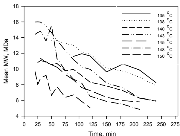
Fig. 3. Change of the mean molecular weight of the obtained water soluble starch derivatives
