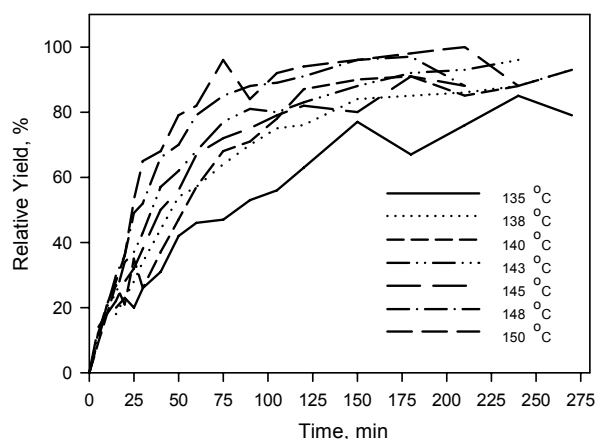
Fig. 2. Variation of the water soluble product yield in function of time at various temperatures
