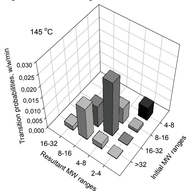
Fig.6. Example for the transition probabilities between different molecular weight categories determined by model fitting for 145 °C reaction temperature
