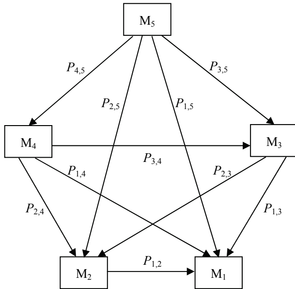
Fig. 1. Principle of the applied mathematical model.
