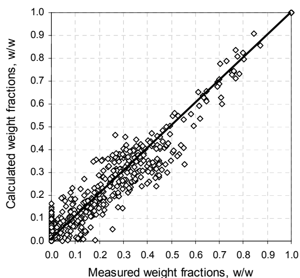
Fig.5. Comparison of the measured and calculated weight fractions obtained by fitting the model
